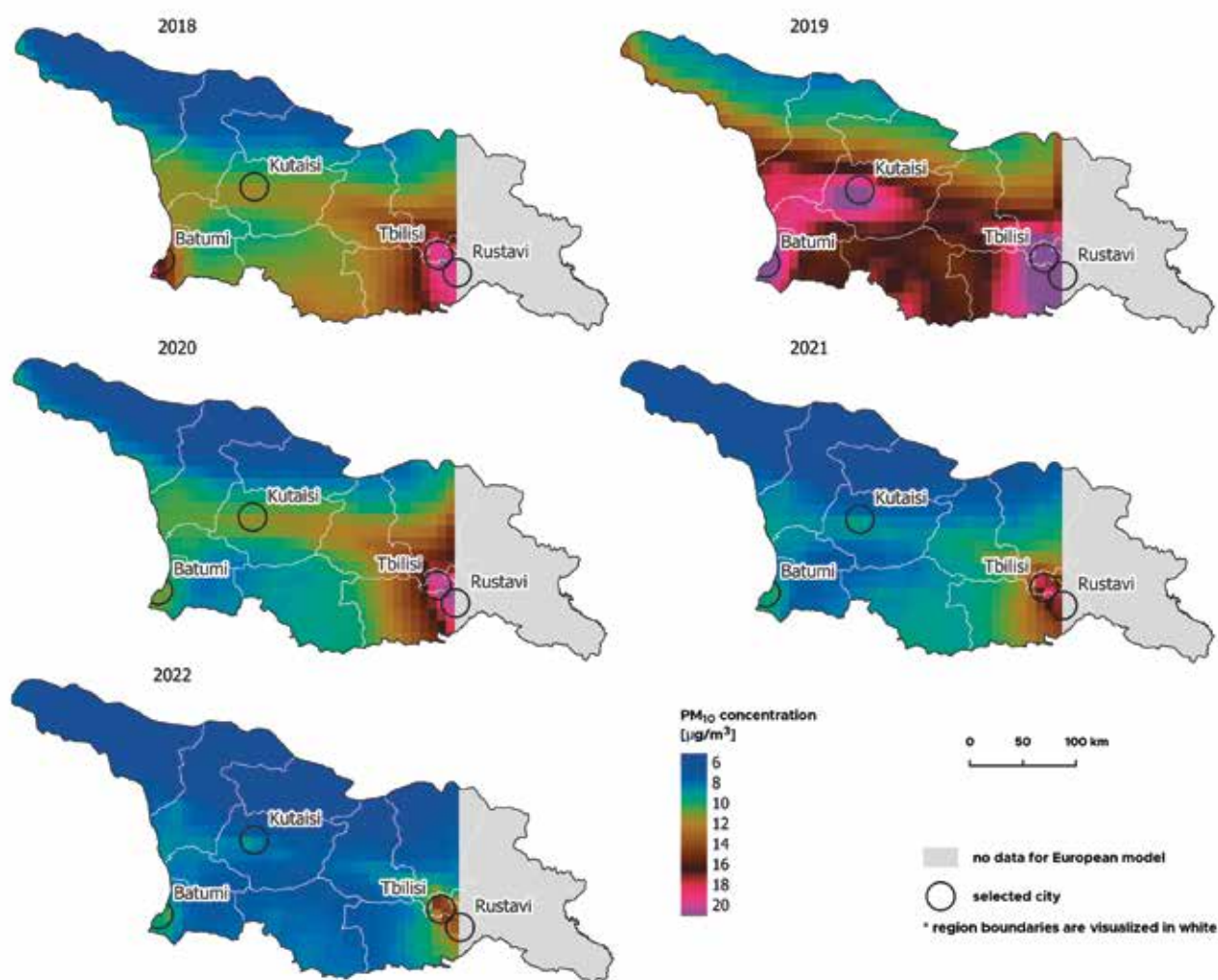
Fig. 31: Average yearly PM_{10} concentrations in Georgia (using the European model) between May 2018 and December 2022, as obtained from the Copernicus Atmosphere Monitoring Service data. Source: CAMS, 2018-2022.
