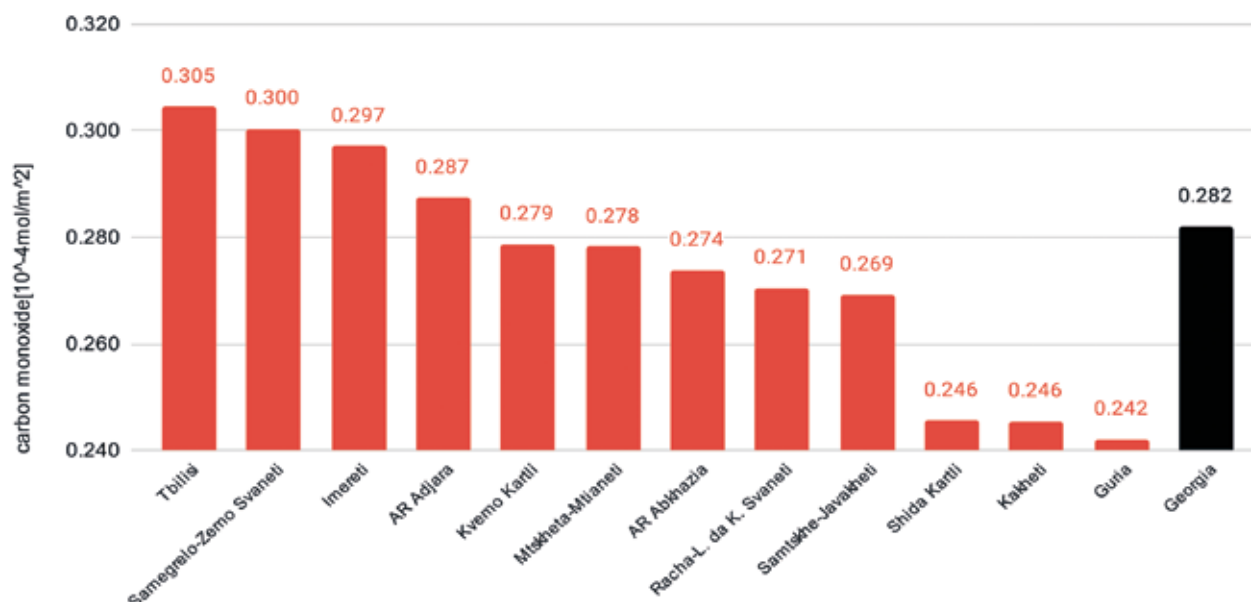
Fig. 21: Average CO concentrations in the regions of Georgia between May 2018 and December 2022, obtained from the Sentinel-5P satellite. Source: ESA, 2018-2020; modified.
