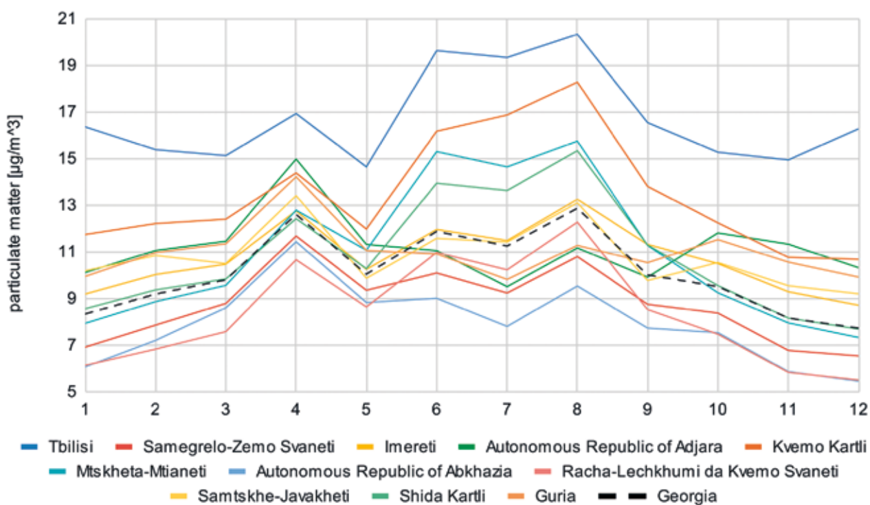
Fig. 35: Seasonality of PM_{10} in the regions of Georgia (using the European model) between May 2018 and December 2022, obtained from the Copernicus Atmosphere Monitoring Service data. Source: CAMS, 2018–2022.
