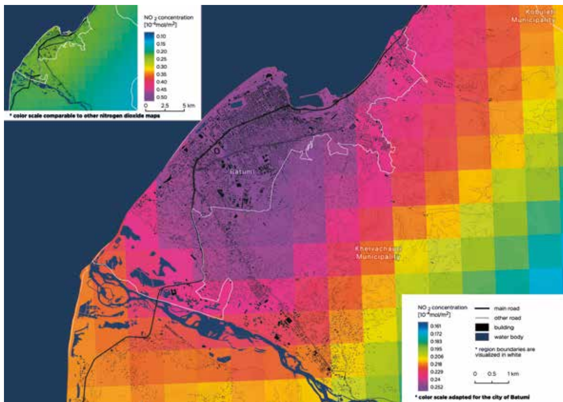
Fig. 13: Average \text{NO}_2 concentrations in Batumi between May 2018 and December 2022, obtained from the Sentinel-5P satellite. Sources: imagery (ESA, 2018–2022; modified), topography (OpenStreetMap Contributors, 2022). Note: Colour scale in the main map adapted to the city of Batumi.
