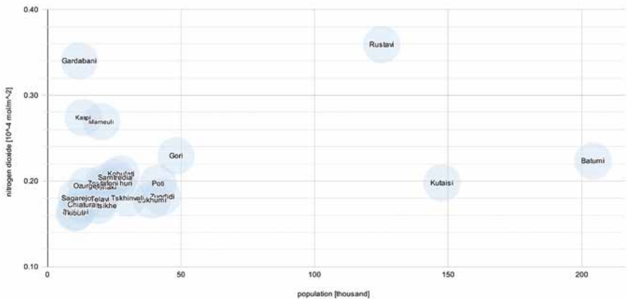
Fig. 11: Average \text{NO}_2 concentrations between May 2018 and December 2022 in the cities in Georgia with a population over 10,000, obtained from the Sentinel-5P satellite. Source: ESA, 2018–2020; modified. Note: Tbilisi is not included in the graph.
