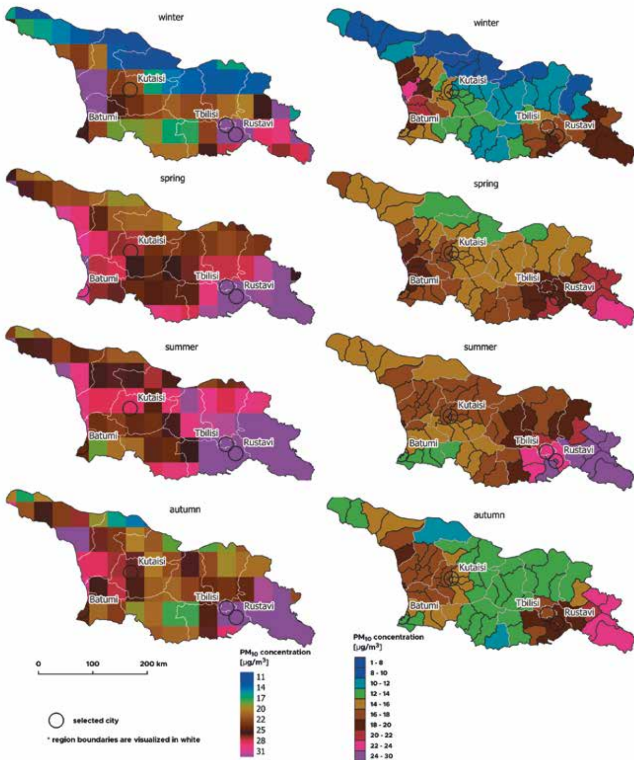
Fig. 32: Average seasonal PM_{10} concentrations in Georgia (using the global model) between May 2018 and December 2022, obtained from the Copernicus Atmosphere Monitoring Service data. Source: CAMS, 2018-2022.
