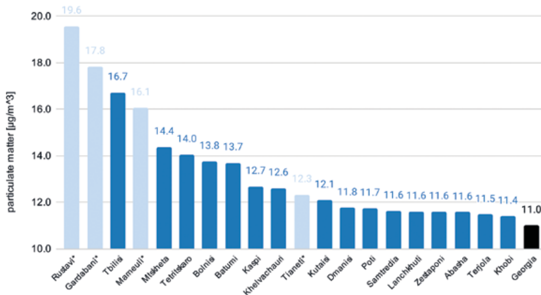
Fig. 29: 20 highest average PM 10 concentrations in municipalities and self-governing cities of Georgia (using the European model) between May 2018 and December 2022, obtained from Copernicus Atmosphere Monitoring Service data. Source: CAMS, 2018-2022. Note (*): The values for the self-governing city of Rustavi and the Gardabani, Tianeti, and Marneuli municipalities do not cover their entire areas.
