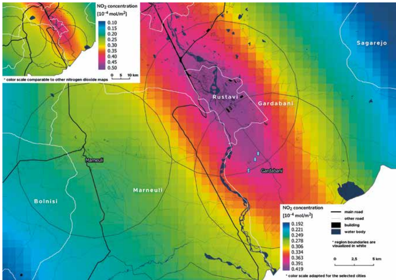
Fig. 15: Average NO 2 concentrations in the agglomeration of Rustavi, Gardabani, and Marneuli between May 2018 and December 2022, obtained from the Sentinel-5P satellite. Sources: imagery (ESA, 2018–2022; modified), topography (OpenStreetMap Contributors, 2022). Note: Colour scale in the main map adapted to the cities of Rustavi, Gardabani, and Marneuli.
