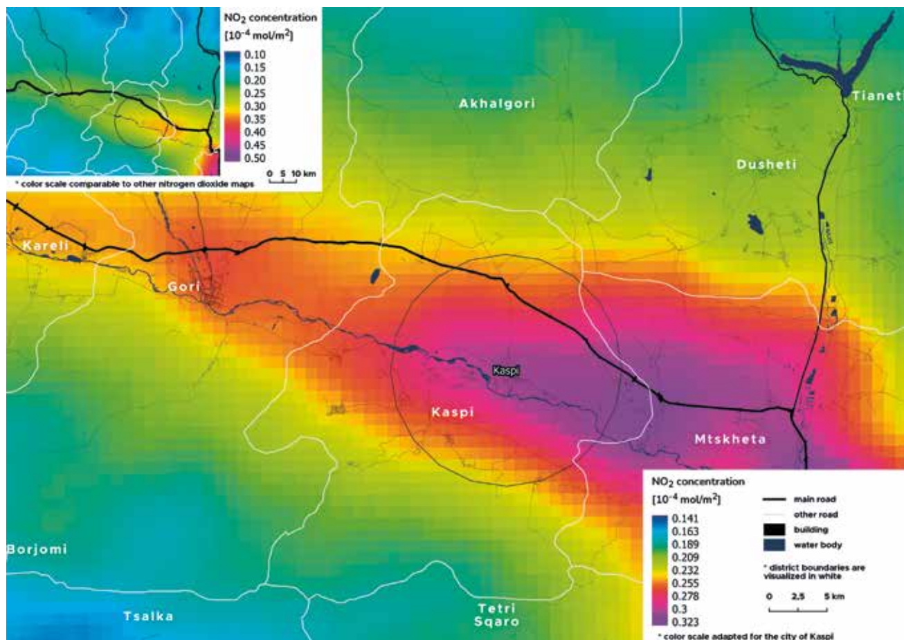
Fig. 16: Average \text{NO}_2 concentrations in Kaspı between May 2018 and December 2022, obtained from the Sentinel-5P satellite. Sources: imagery (ESA, 2018–2022; modified), topography (OpenStreetMap Contributors, 2022). Note: Colour scale adapted for the city of Kaspı.
