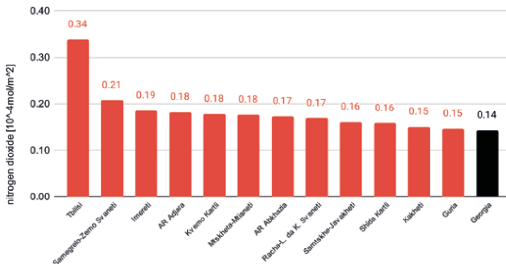
Fig. 6: Average NO 2 concentrations in the regions of Georgia between May 2018 and December 2022, obtained from the Sentinel-5P satellite. Source: ESA, 2018–2020; modified.
