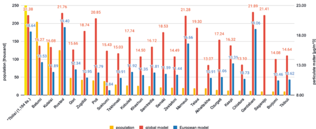
Fig. 36: Average PM_{10} concentrations in cities with a population over 10,000 in Georgia between May 2018 and December 2022, obtained from the Copernicus Atmosphere Monitoring Service data. Source: CAMS, 2018-2022.
