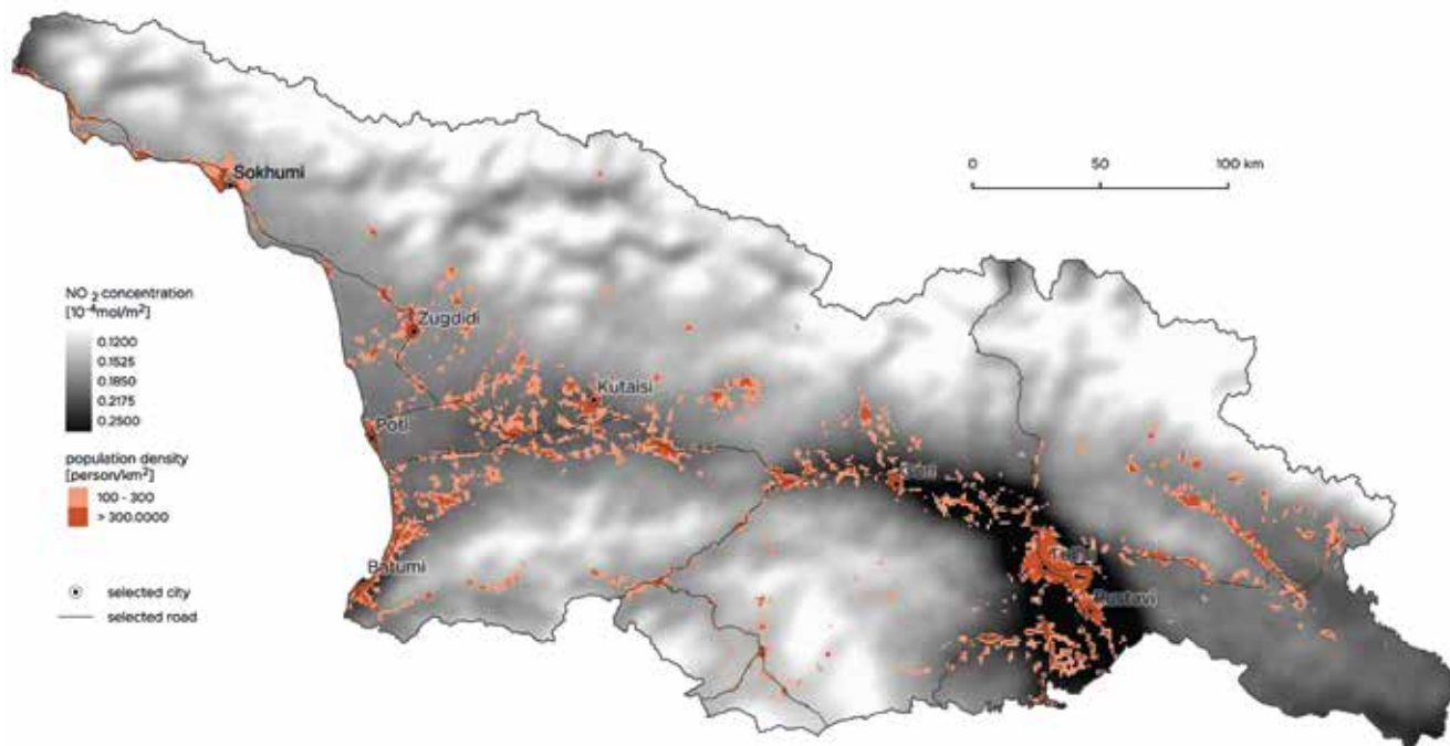
Fig. 17: Average \text{NO}_2 concentrations in Georgia between May 2018 and July 2020, obtained from the Sentinel-5P satellite in context with the 2019 population density data. Sources: imagery (ESA, 2018-2020; modified), topography (OpenStreetMap Contributors, 2022), population (WorldPop, 2020).
