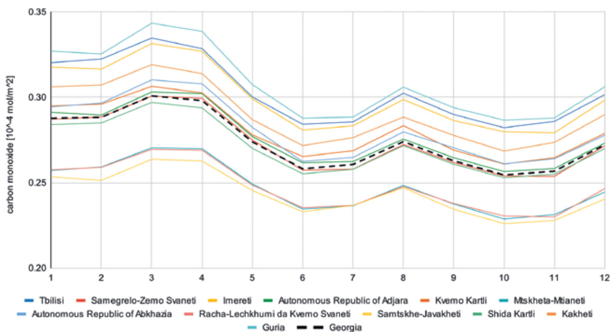
Fig. 24: Average monthly CO concentrations in the regions of Georgia between May 2018 and December 2022, obtained from the Sentinel-5P satellite. Source: ESA, 2018-2020; modified.
