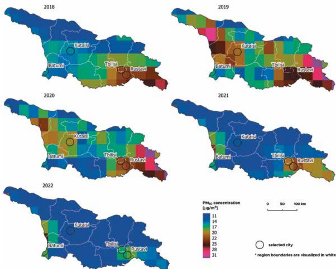
Fig. 30: Average yearly PM 10 concentrations in Georgia (using the global model) between May 2018 and December 2022, obtained from the Copernicus Atmosphere Monitoring Service data. Source: CAMS, 2018-2022.
