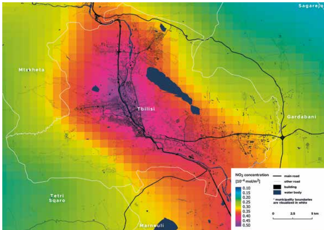
Fig. 12: Average \text{NO}_2 concentrations in Tbilisi between May 2018 and December 2022, obtained from the Sentinel-5P satellite. Sources: imagery (ESA, 2018–2022; modified), topography (OpenStreetMap Contributors, 2022).
