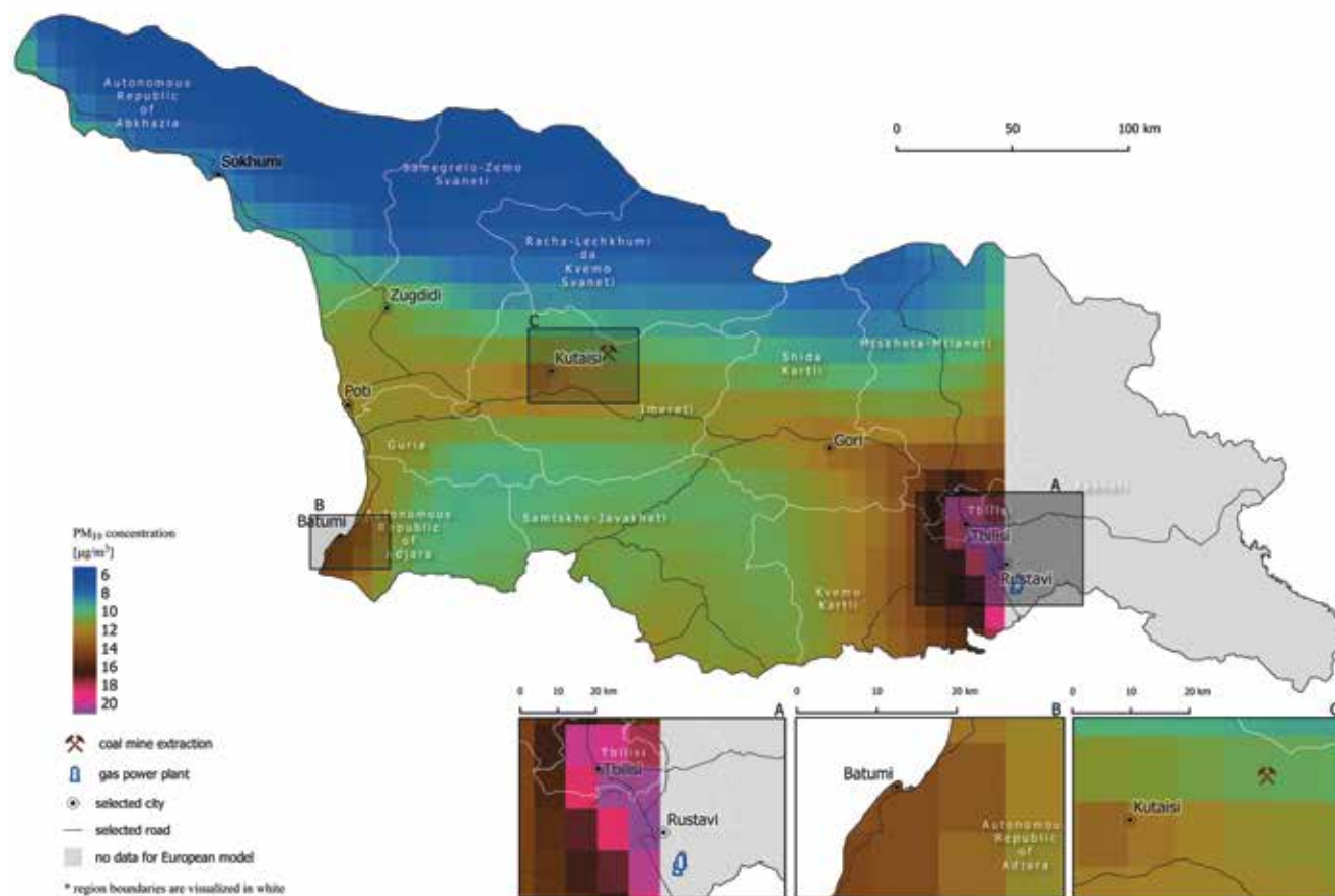
Fig. 26: Average PM_{10} concentrations in Georgia (European model) between May 2018 and December 2022, obtained from the Copernicus Atmosphere Monitoring Service data. Sources: CAMS, 2018-2022; topography (OpenStreetMap Contributors, 2022), coal and gas (Global Energy Monitor, 2023).
