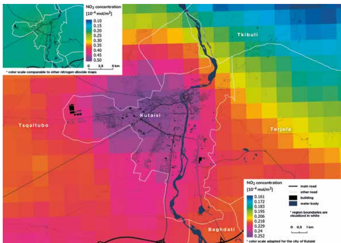
Fig. 14: Average \text{NO}_2 concentrations in Kutaisi between May 2018 and December 2022, obtained from the Sentinel-5P satellite. Sources: imagery (ESA, 2018–2022; modified), topography (OpenStreetMap Contributors, 2022). Note: Colour scale in the main map adapted to the city of Kutaisi.
