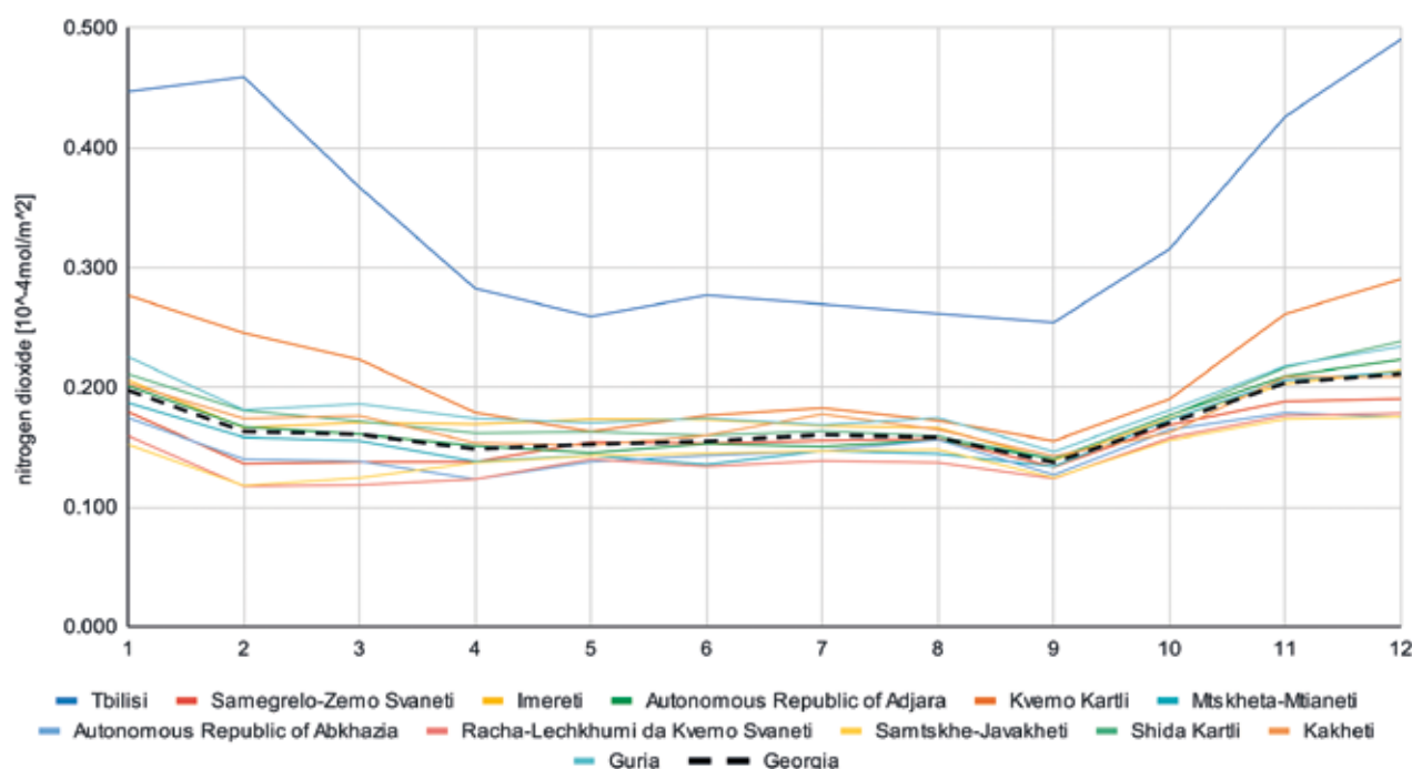
Fig. 9: Average monthly \text{NO}_2 concentrations in the regions of Georgia between May 2018 and December 2022, obtained from the Sentinel-5P satellite. Source: ESA, 2018-2020; modified.
