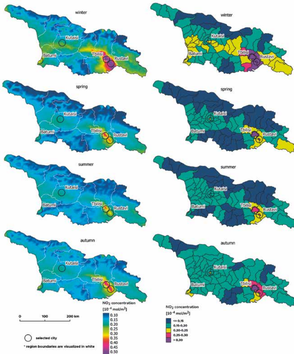
Fig. 8: Average seasonal \text{NO}_2 concentrations in the regions of Georgia between May 2018 and December 2022, obtained from the Sentinel-5P satellite. Source: ESA, 2018-2020; modified.
