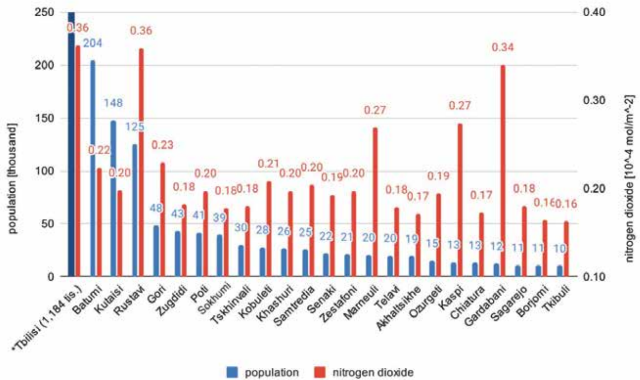
Fig. 10: Average \text{NO}_2 concentrations between May 2018 and December 2022 in the cities of Georgia with a population over 10,000, obtained from the Sentinel-5P satellite. Source: ESA, 2018–2020; modified.
