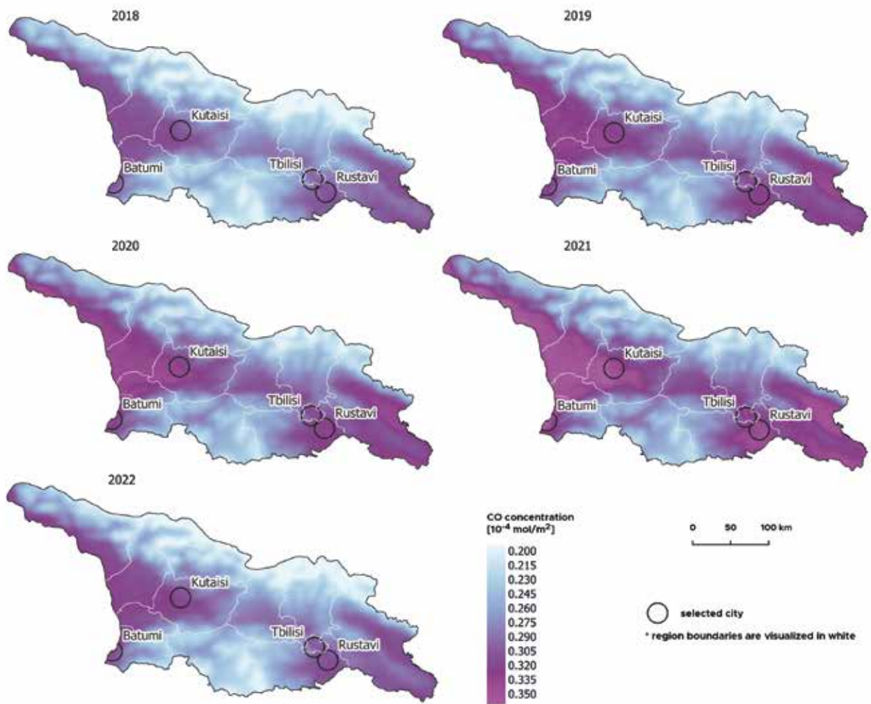
Fig. 20: Average yearly CO concentrations in Georgia between May 2018 and December 2022, obtained from the Sentinel-5P satellite. Sources: ESA, 2018-2020; modified.
