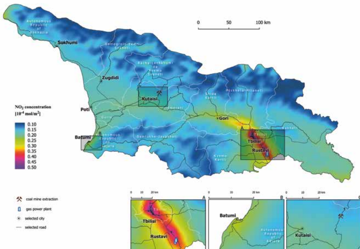
Fig. 4: Average \text{NO}_2 concentrations in Georgia between May 2018 and December 2022, obtained from the Sentinel-5P satellite. Sources: imagery (ESA, 2018-2022; modified), roads and cities (OpenStreetMap Contributors, 2022), coal and gas (Global Energy Monitor, 2023).
