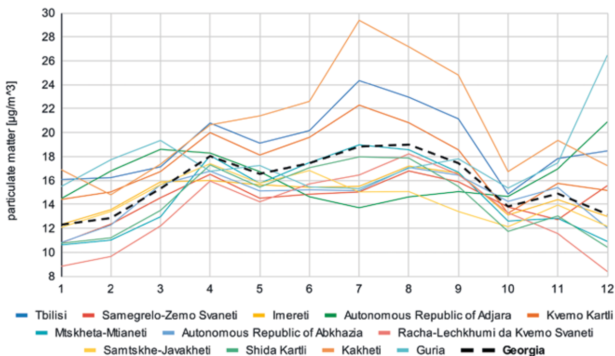
Fig. 34: Seasonality of PM_{10} in the regions of Georgia (using the global model) between May 2018 and December 2022, obtained from the Copernicus Atmosphere Monitoring Service data. Source: CAMS, 2018–2022.
