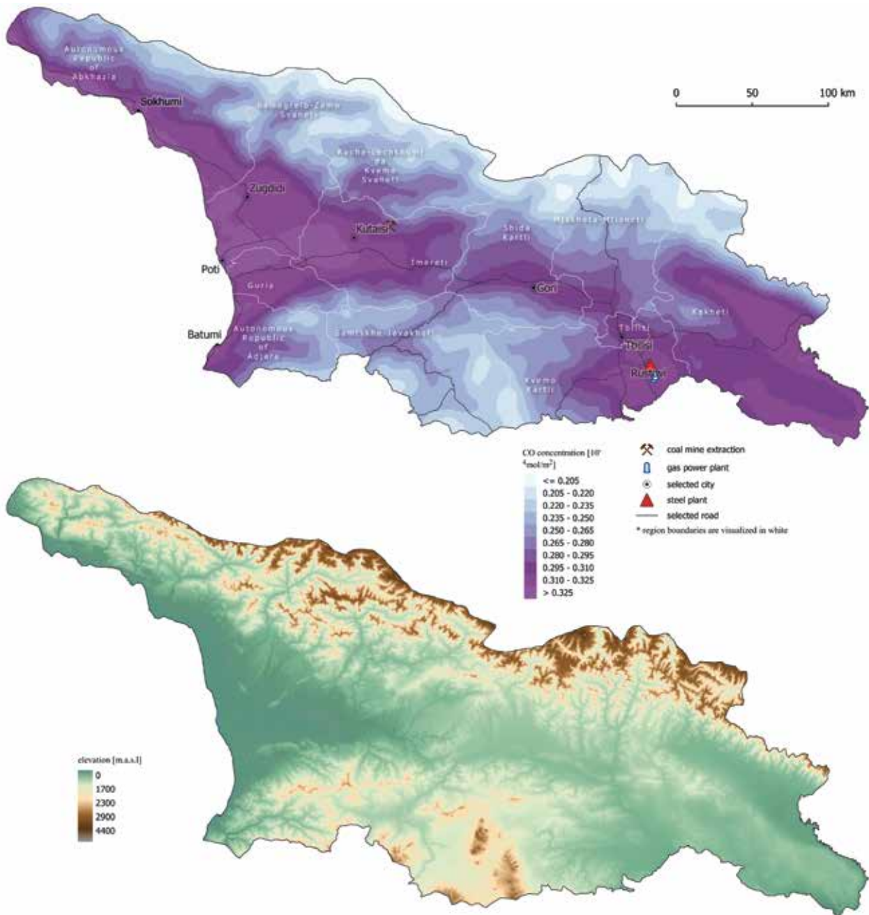
Fig. 19: Average CO concentrations in Georgia between May 2018 and December 2022, obtained from the Sentinel-5P satellite in context with a digital elevation model. Sources: imagery (ESA, 2018-2020; modified), roads (OpenStreetMap Contributors, 2022; modified), elevation (USGS, 2023).
