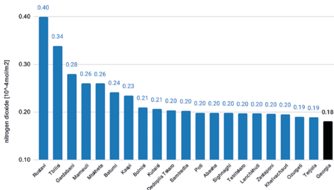
Fig. 7: 20 highest average NO 2 concentrations in municipalities and self-governing cities of Georgia between May 2018 and December 2022, obtained from the Sentinel-5P satellite. Source: ESA, 2018–2020; modified.
