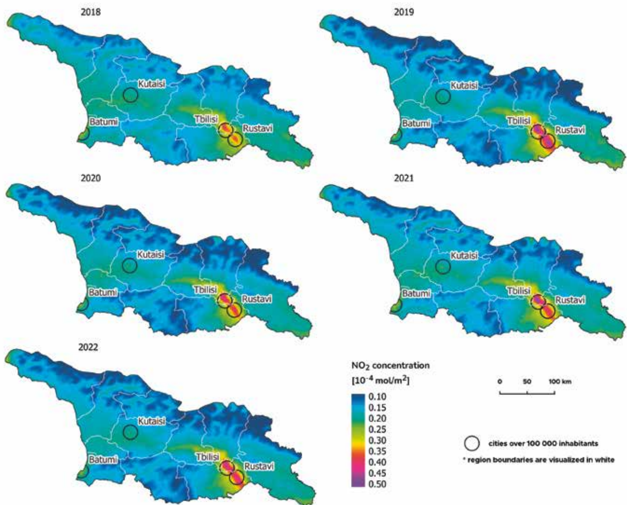
Fig. 5: Average yearly \text{NO}_2 concentrations in Georgia between May 2018 and December 2022, obtained from the Sentinel-5P satellite. Sources: ESA, 2018-2020; modified.
