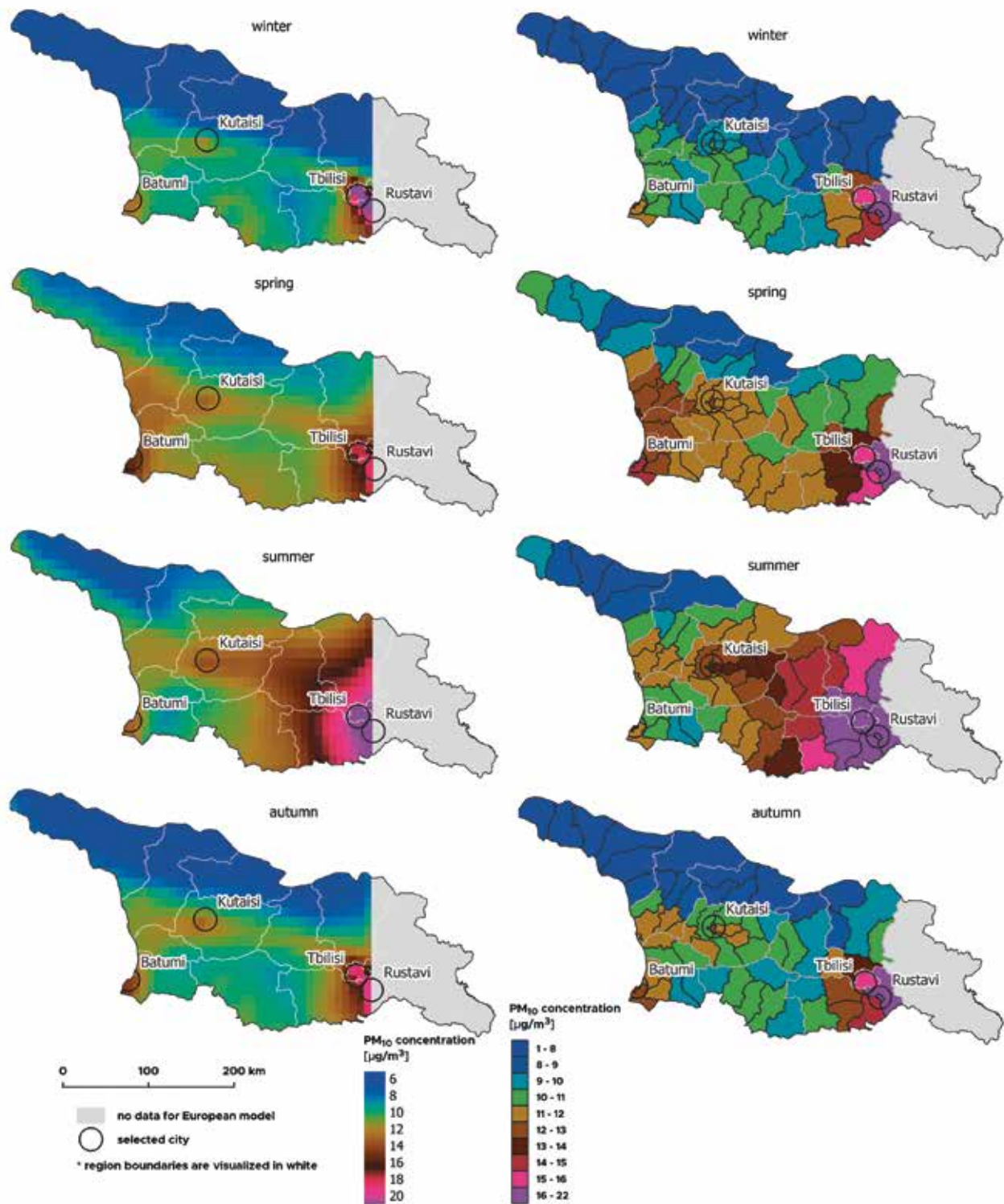
Fig. 33: Average seasonal PM 10 concentrations in the regions of Georgia (using the European model) between May 2018 and December 2022, as obtained from the Copernicus Atmosphere Monitoring Service data. Source: CAMS, 2018-2022.
