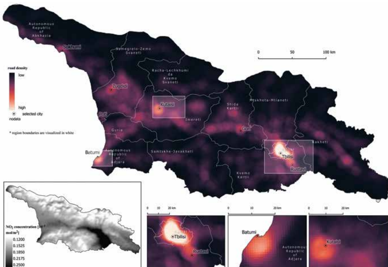
Fig. 18: Average \text{NO}_2 concentrations in Georgia between May 2018 and July 2020 (bottom left corner) in context with road density (main map). Sources: imagery (ESA, 2018-2020; modified), roads (OpenStreetMap Contributors, 2022; modified).
