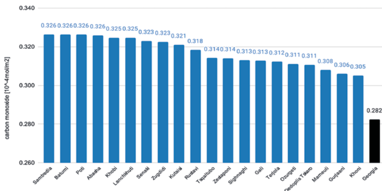
Fig. 22: 20 highest average CO concentrations in municipalities and self-governing cities of Georgia between May 2018 and December 2022, obtained from the Sentinel-5P satellite. Source: ESA, 2018-2020; modified.
