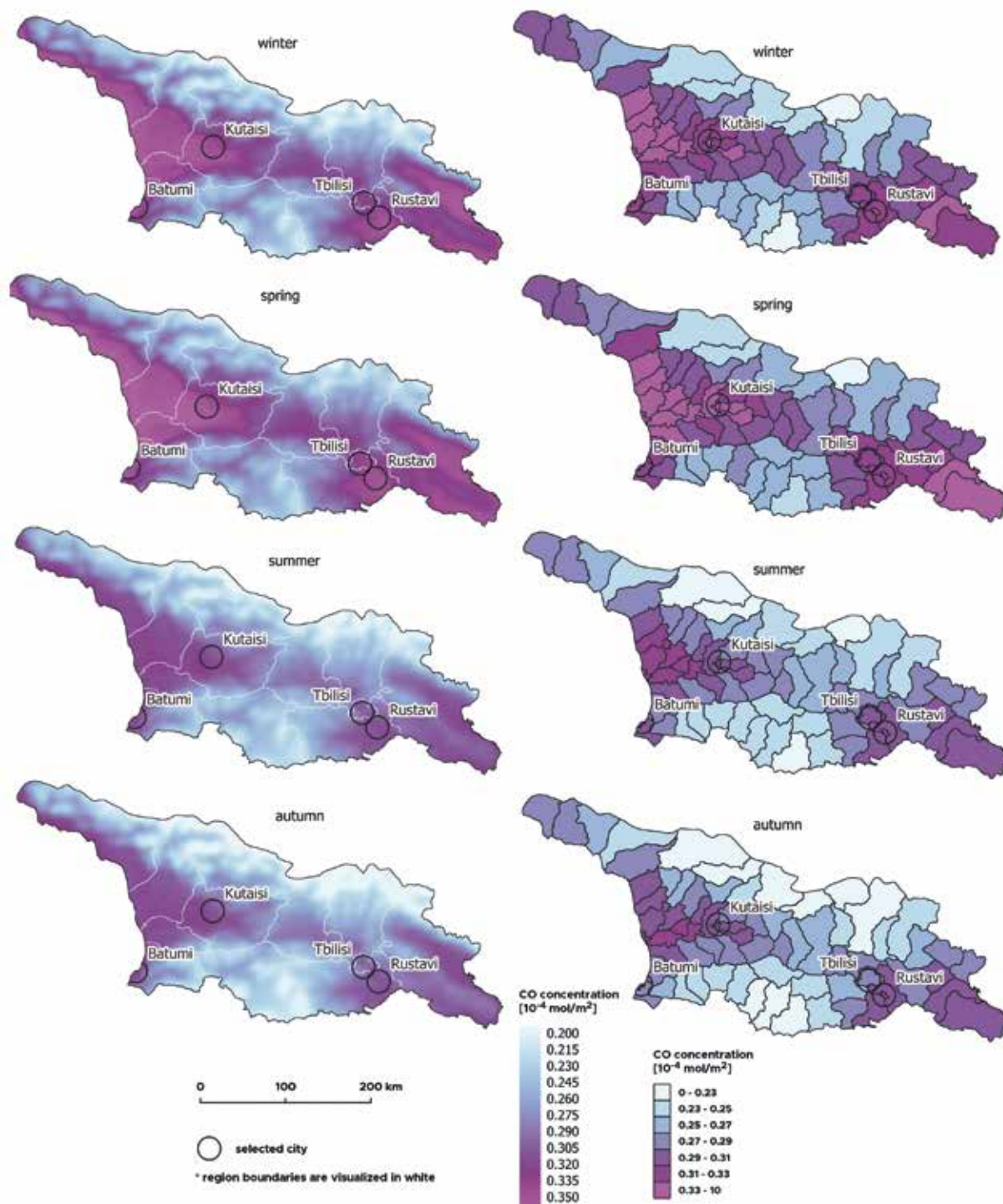
Fig. 23: Average seasonal CO concentrations in the regions of Georgia between May 2018 and December 2022, obtained from the Sentinel-5P satellite. Source: ESA, 2018-2020; modified.
