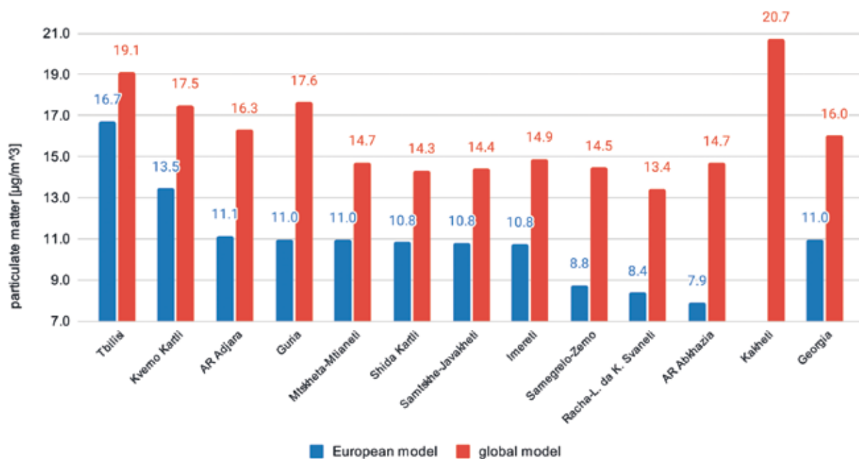
Fig. 27: Average PM_{10} concentrations in the regions of Georgia between May 2018 and December 2022, obtained from the Copernicus Atmosphere Monitoring Service data. Source: CAMS, 2018-2022.
