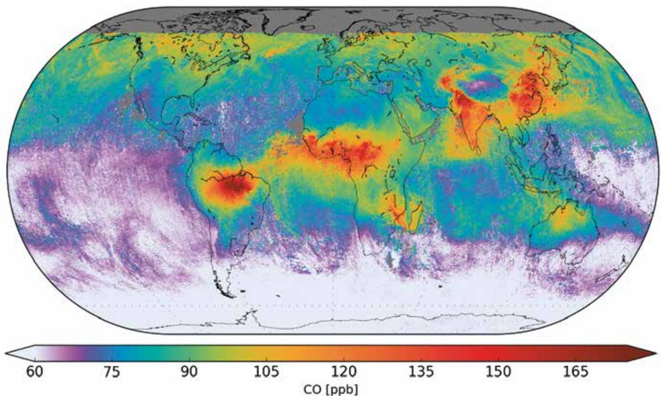
Fig. 2: The global CO total column mixing ratio average concentration created with TROPOMI L2 data (November 13th-19th 2017), The data clearly shows CO enhancement by wildfires in Brazil, Africa, Madagascar, and Australia as well as anthropogenic air pollution in India and China). Source: TROPOMI, 2023.
