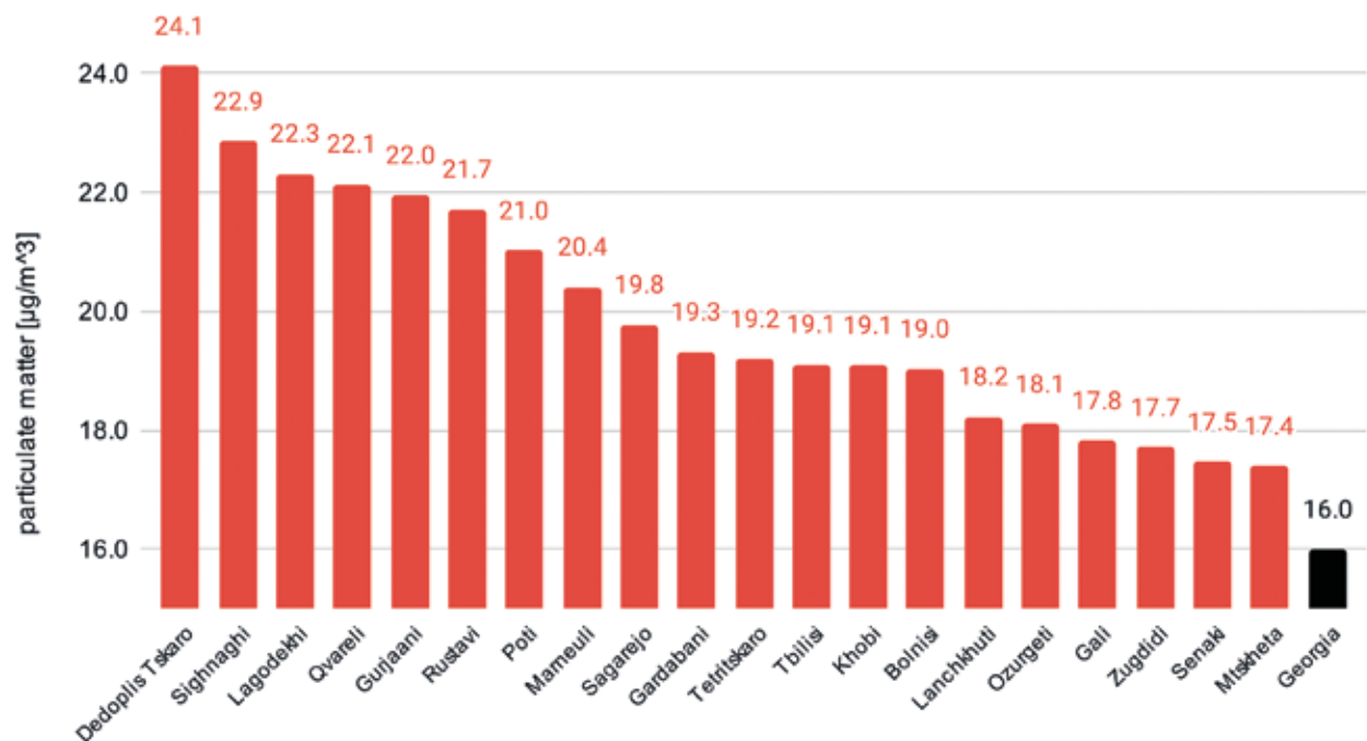
Fig. 28: 20 highest average PM_{10} concentrations in municipalities and self-governing cities of Georgia (using the global model) between May 2018 and December 2022, obtained from Copernicus Atmosphere Monitoring Service data. Source: CAMS, 2018-2022.
